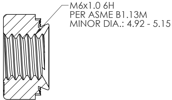
SECTION A-A SCALE 3.5 : 1
